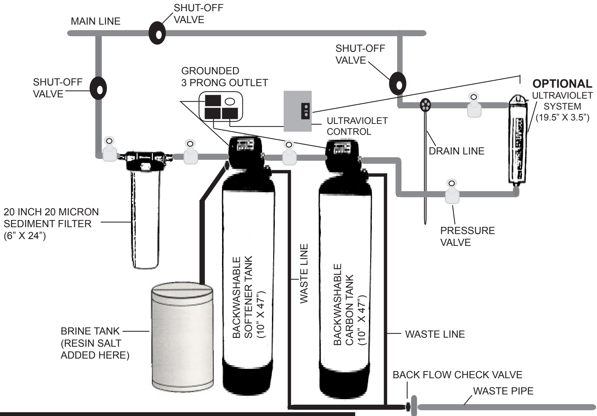
WHOLE HOUSE FILTRATION SYSTEM SYSTEM 3 (CARBON TANK & SOFTENER TANK & SEDIMENT FILTER & ULTRAVIOLET)
