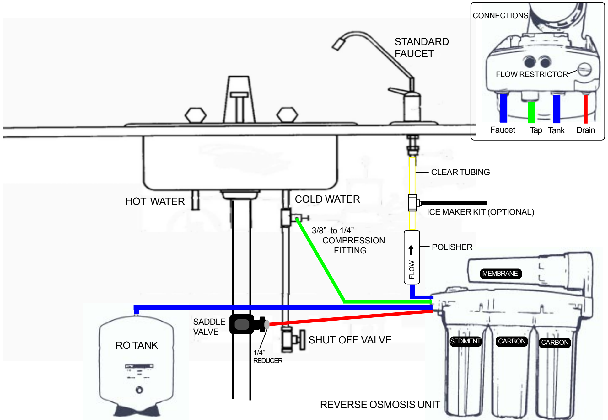
REVERSE OSMOSIS WITH STANDARD FAUCET
