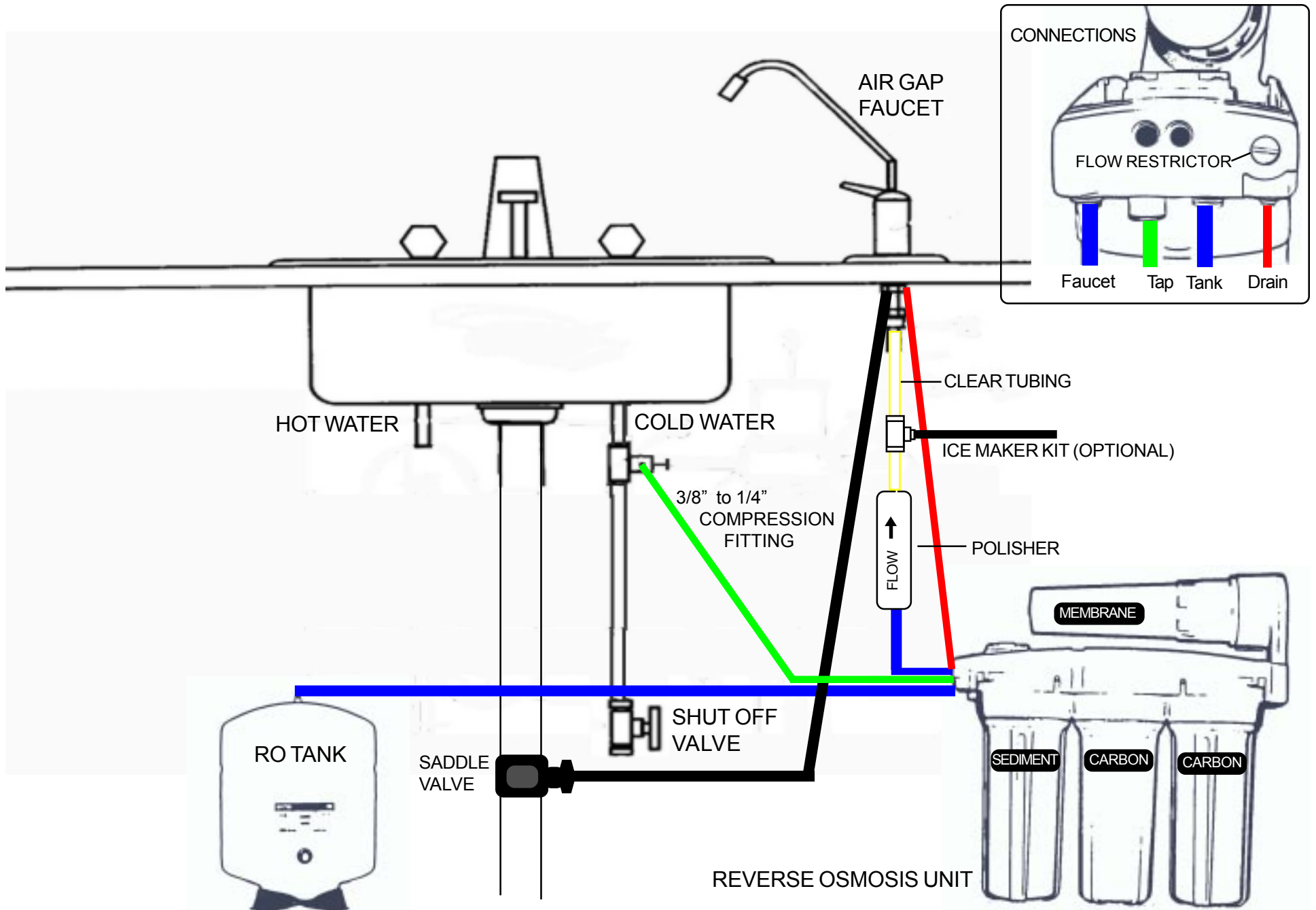
REVERSE OSMOSIS WITH AIR GAP FAUCET
